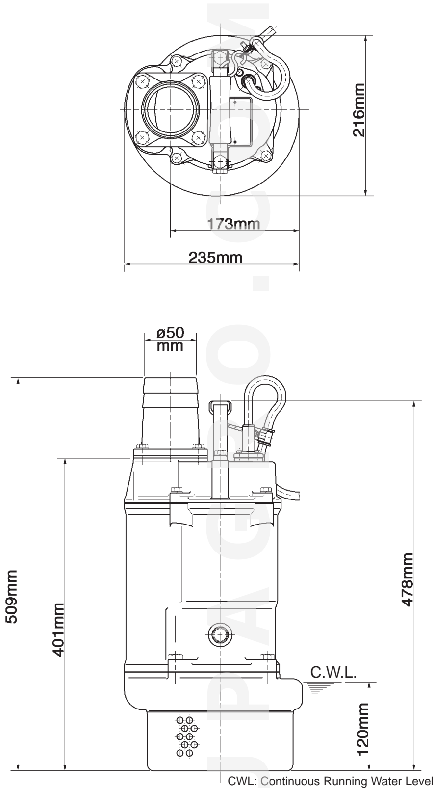
CWL: Continuous Running Water Level KTZ21.5-51 (A-10127-1)
