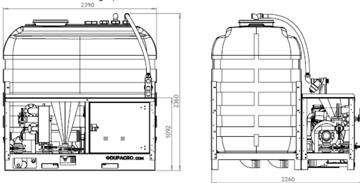
M5D-S4 Enkel tank afmetingen; 2390x2260x2360mm
