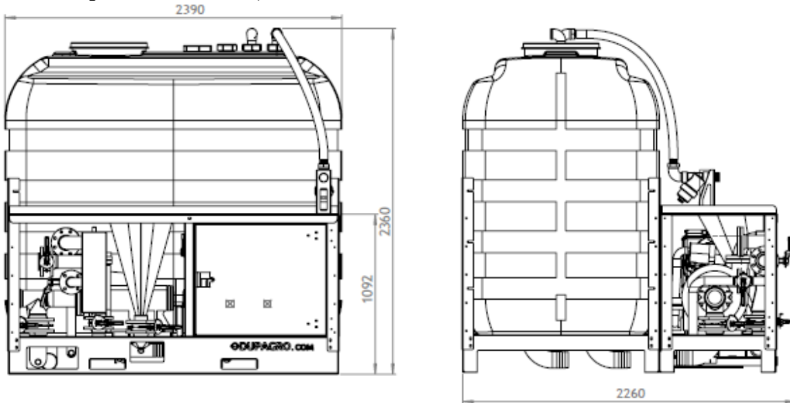
M5D-S3 Single Tank Dimensions; 2390x2260x2360mm
