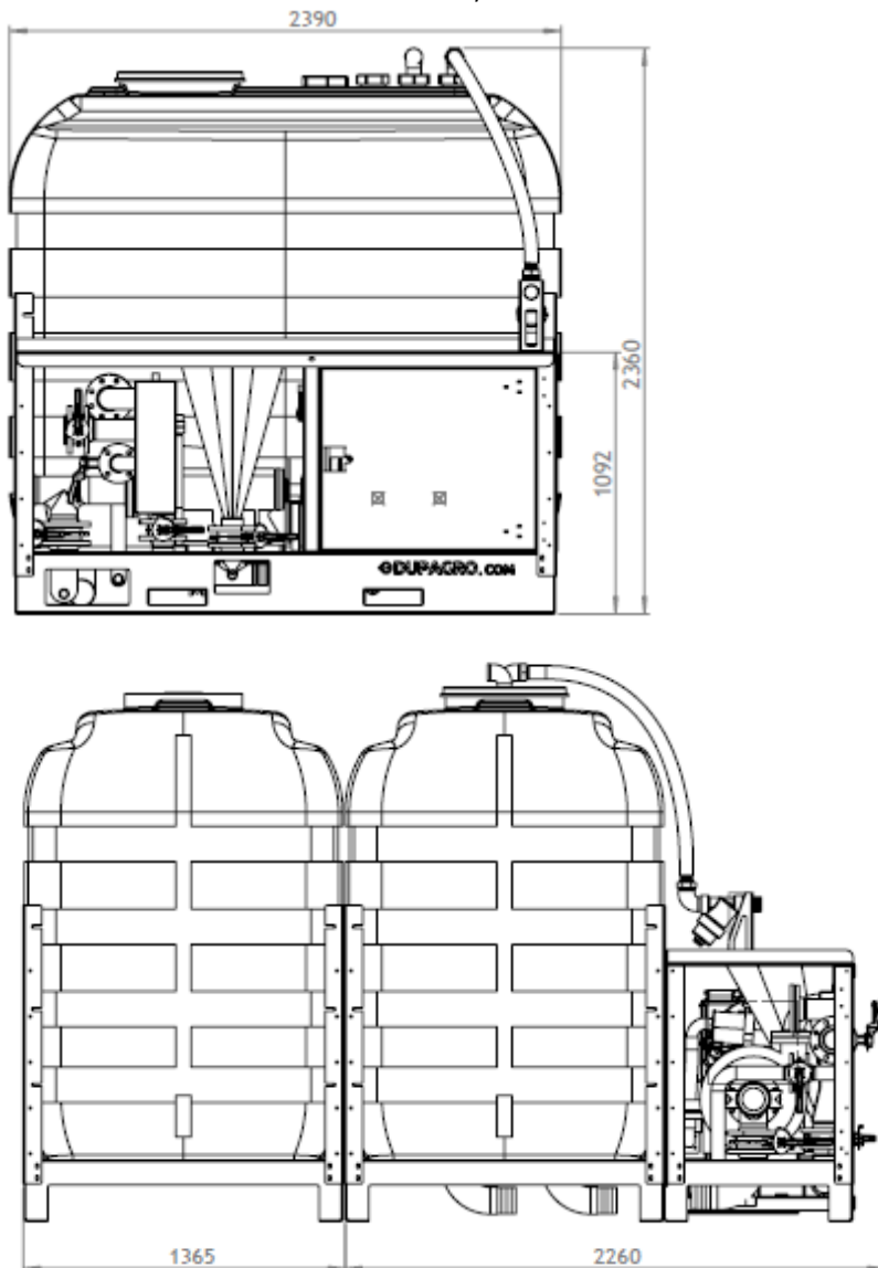
M5D-S3-2M Double Tank Dimensions; 2390x3625x2360mm
