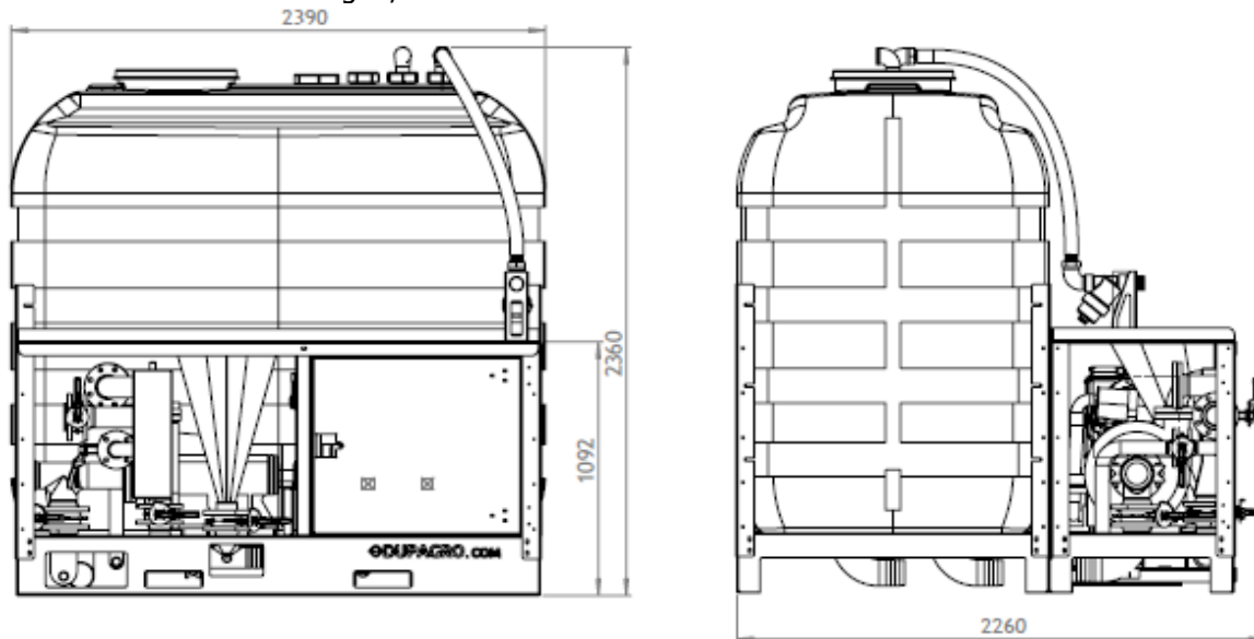
M5E-S4 Enkel tank afmetingen; 2390x2260x2360mm
